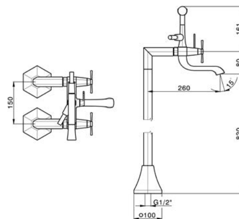
CX004200 Completo Miscelatore Vasca Free-Standing Free-Standing Bath/S. Mixer Set Ensemble Mélangeur Bain/D. Free-Standing
