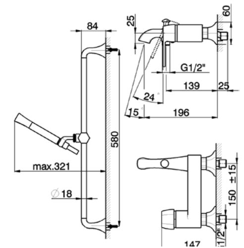
CH000064 Completo Monocomando Vasca Bath/S. Mixer Set Ensemble Mitigeur Bain/D.
