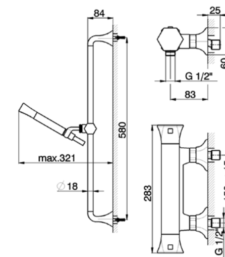
CES01010 Completo Termostatico Doccia Thermo Shower Set Ensemble Thermo Douche
