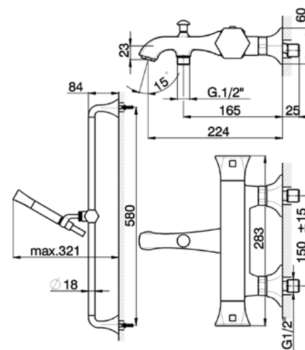
CES27010 Completo Termostatico Vasca Thermo Bath/S. Set Ensemble Thermo Bain/D.
