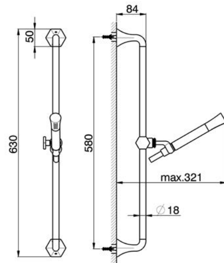
CE003110 Completo Doccia Saliscendi 580mm 580mm Slide Rail Shower Set Ensemble Barre de Douche 580mm
