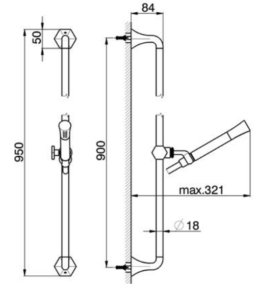
CE003111 Completo Doccia Saliscendi 900mm 900mm Slide Rail Shower Set Ensemble Barre de Douche 900mm
