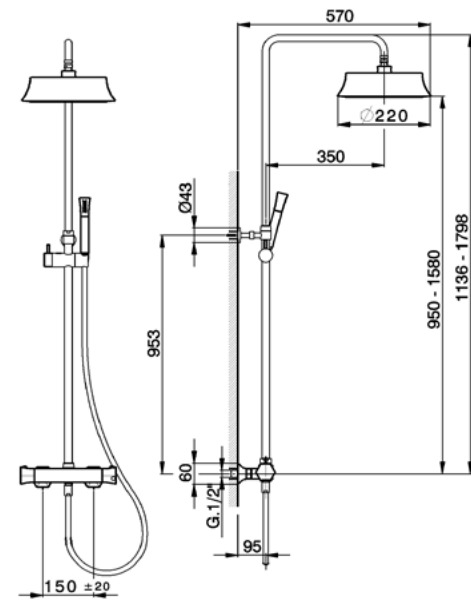
CEC82010 CombiDoccia Termostatico Thermo CombiShower CombiDouche Thermo
