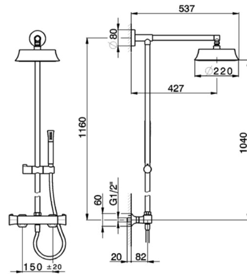
CEC78010 CombiDoccia Termostatico Thermo CombiShower CombiDouche Thermo
