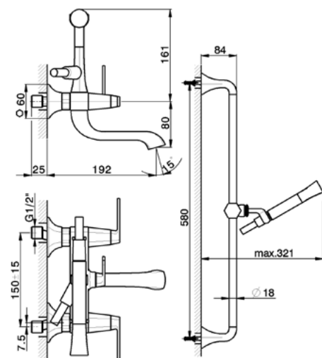
CF000060 Completo Miscelatore Vasca Bath/S. Mixer Set Ensemble Mélangeur Bain/D.
