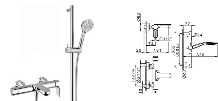
RK 00060 Completo Monocomando Vasca Mixer Bath/S. Set Ensemble Mitigeur Bain/D.
